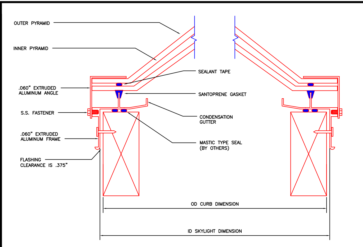
CURB MOUNT PYRAMID (MODEL CM-PYR)
